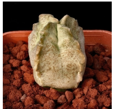
Whitesloanea crassa
